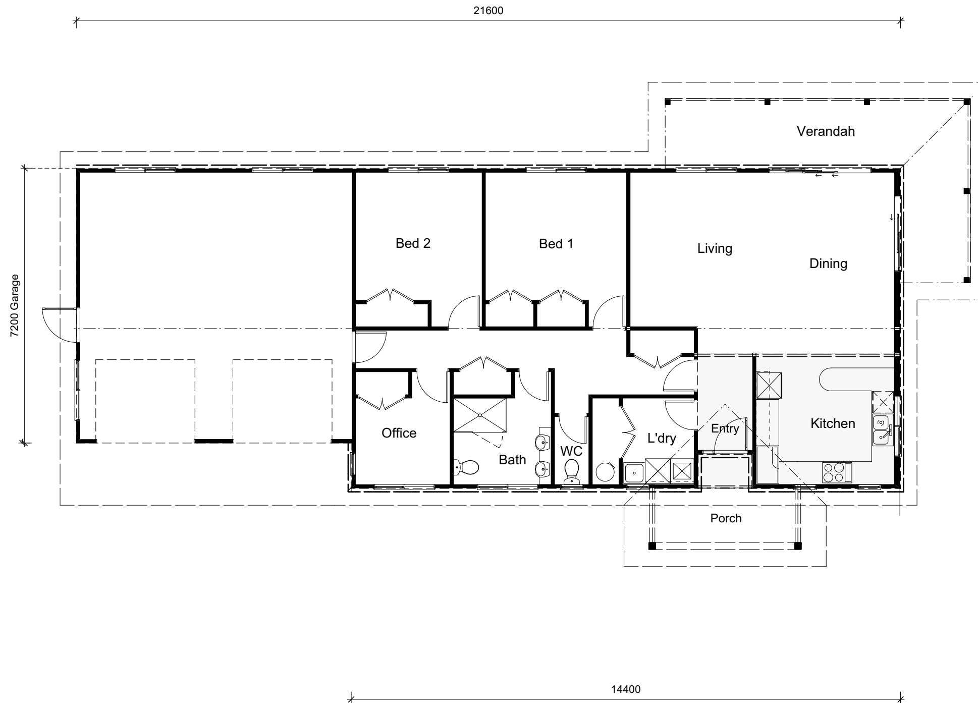
○ FLOOR PLAN
